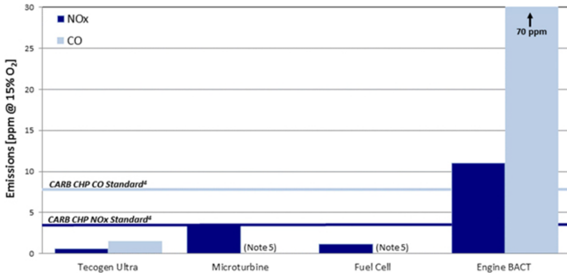
Figure 5 – Comparison of Tecogen Ultra Low-Emissions Technology to Other Technologies
