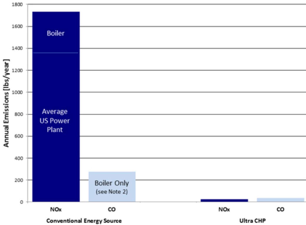
Figure 4 – Comparison of Emissions Levels of Tecogen’s Ultra Low-Emissions Technology to Conventional Energy Sources (Based on 6,000 hrs/year of operation at 100 kW and 670,000 Btu/hr) Source: Tecogen Inc.
