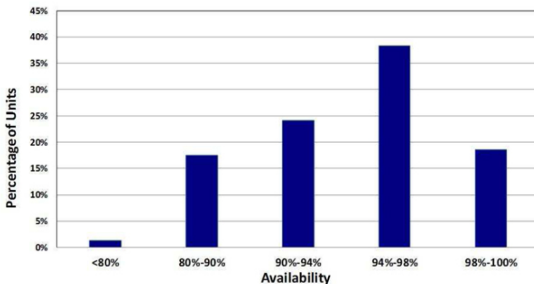
Figure 7 – Tecogen Product Reliability Source: Tecogen Inc.
