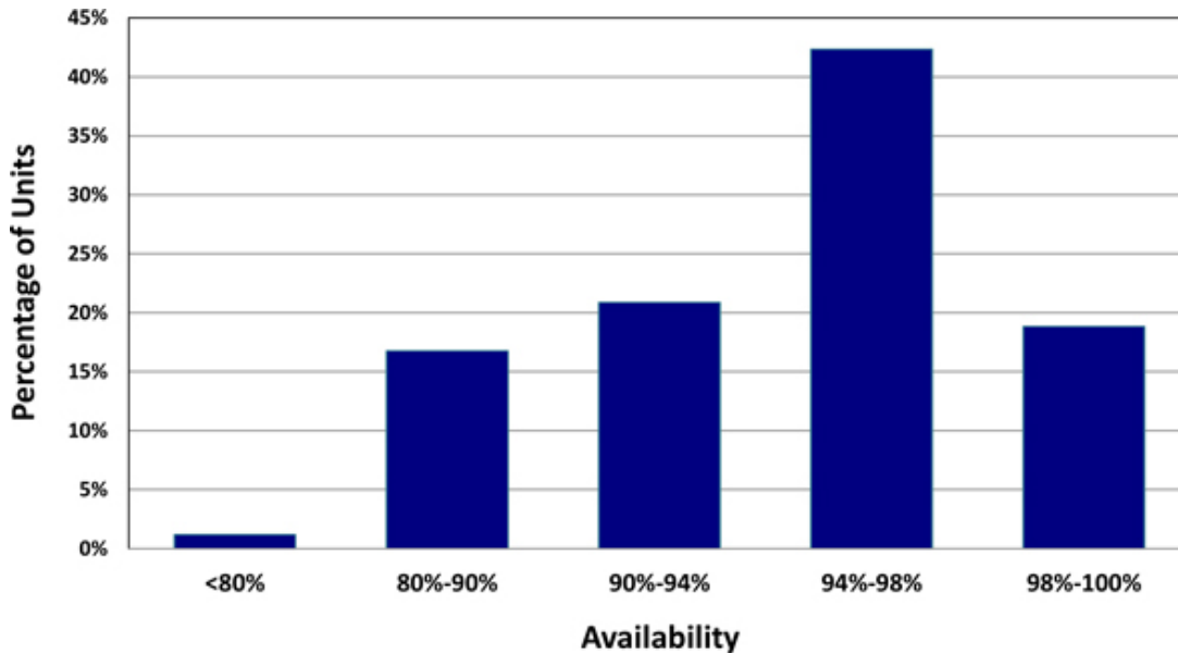
Figure 7 — Tecogen Product Reliability Source: Tecogen Inc. - January 2014
