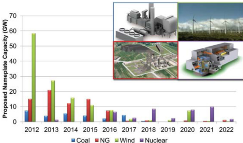
Figure 1 — Proposed U.S. New Capacity: Coal, Natural Gas, Wind, and Nuclear
